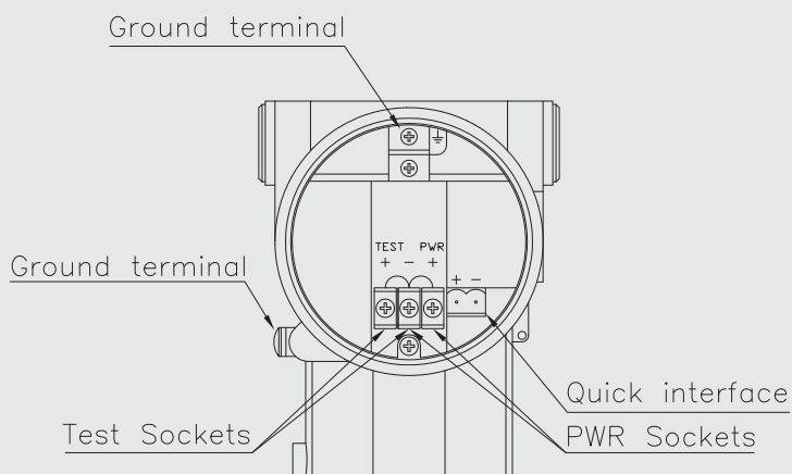
Terminal Configuration
